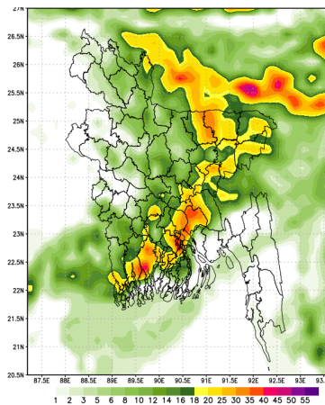
Simulated Rainfall (mm) (WRF model) Period (08-04-2020 to 14-04-2020)
