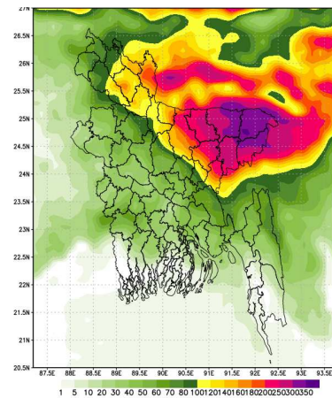
Extended outlook for accumulative rainfall(mm) Period (15-04-2020 to 21-04-2020)
