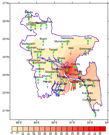
Spatial distribution of Rainfall (mm) Period 01-04-2020 to 07-04-2020
