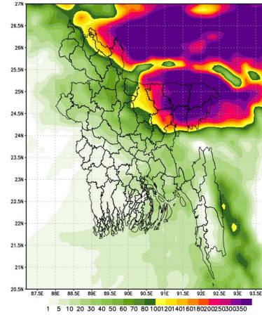
Extended outlook for accumulative rainfall(mm) Period (27-05-2020 to 03-06-2020)
