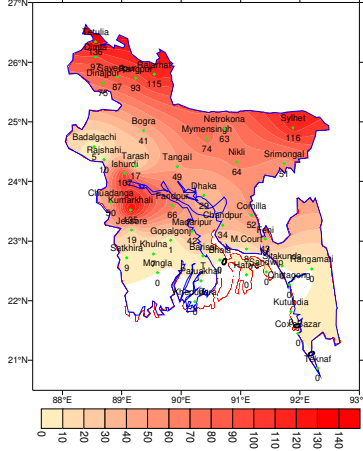
Spatial distribution of Rainfall (mm) Period 10-05-2020 to 16-05-2020
