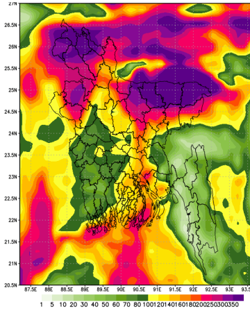
Simulated Rainfall (mm) (WRF model) Period (17-05-2020 to 26-05-2020)
