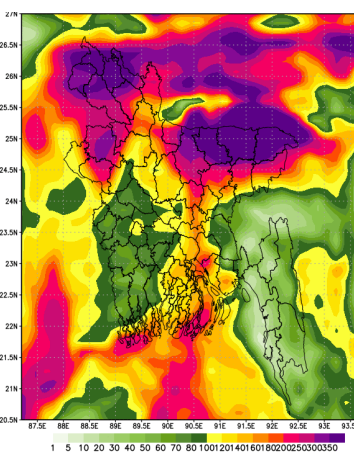
Simulated Rainfall (mm) (WRF model) Period (17-05-2020 to 26-05-2020)
