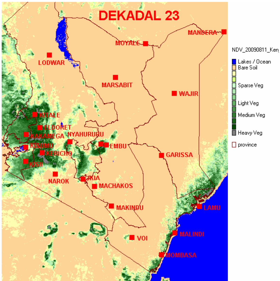
FIG 5: DEKADAL 23 Normalized Difference Vegetation Index (11th to 20th August, 2009)
